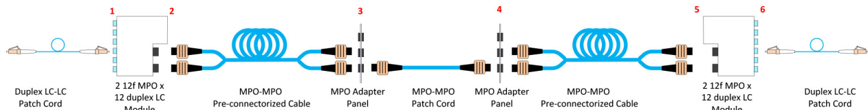
FIGURE 2: Cross Connect with two-trunk link and breakout modules
